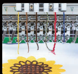
Multi cording Device 2 Embroidering 6 various types/colors of cords
